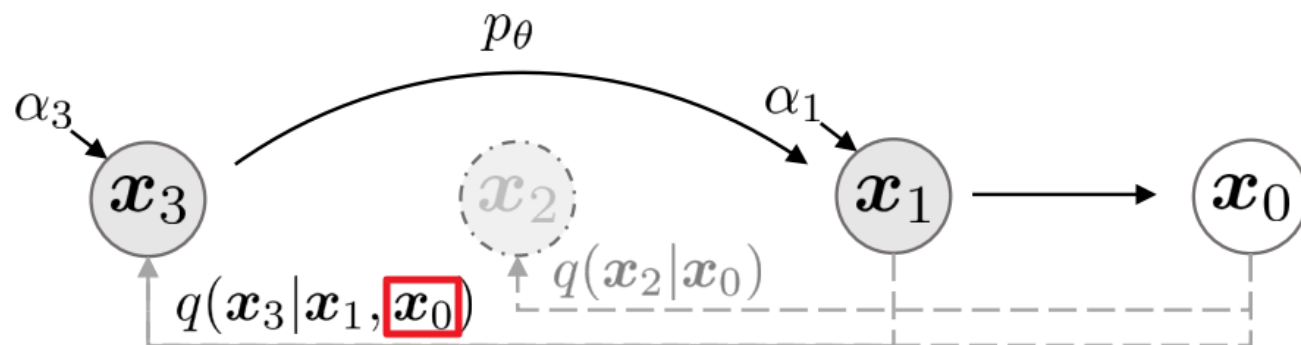
Figure 2: Graphical model for accelerated generation, where \tau = [1, 3] .
